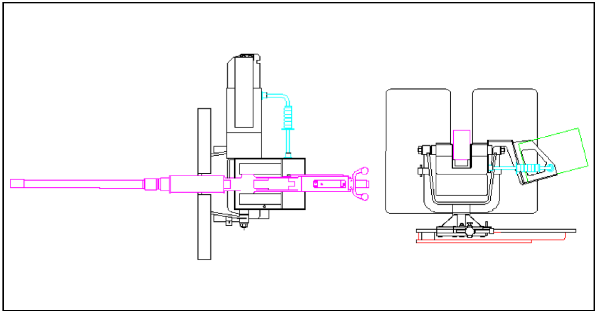
SCHEMATIC SLIDING ARM MACHINE GUN MOUNT
