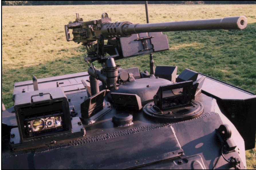
TYPICAL 0.5" HEAVY MACHINE GUN MOUNTED ON A SWINGING ARM PINTLE MOUNT
