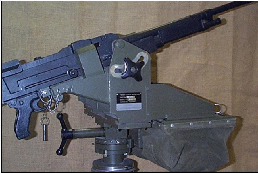
7.62 mm MACHINE GUN MOUNT
